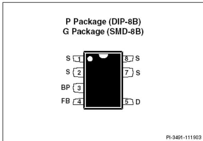
Figure 3. 핀 배열.
