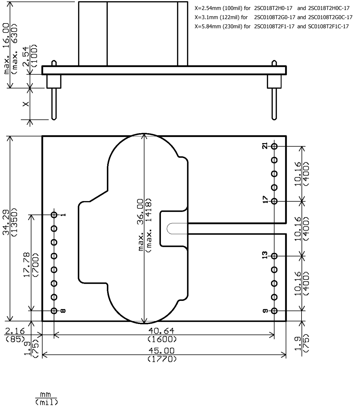
Fig. 4 Mechanical drawing of 2SC0108T
