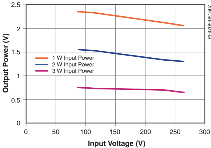
Figure 2. Available Standby Power at 1 W, 2 W and 3 W Input Power.
