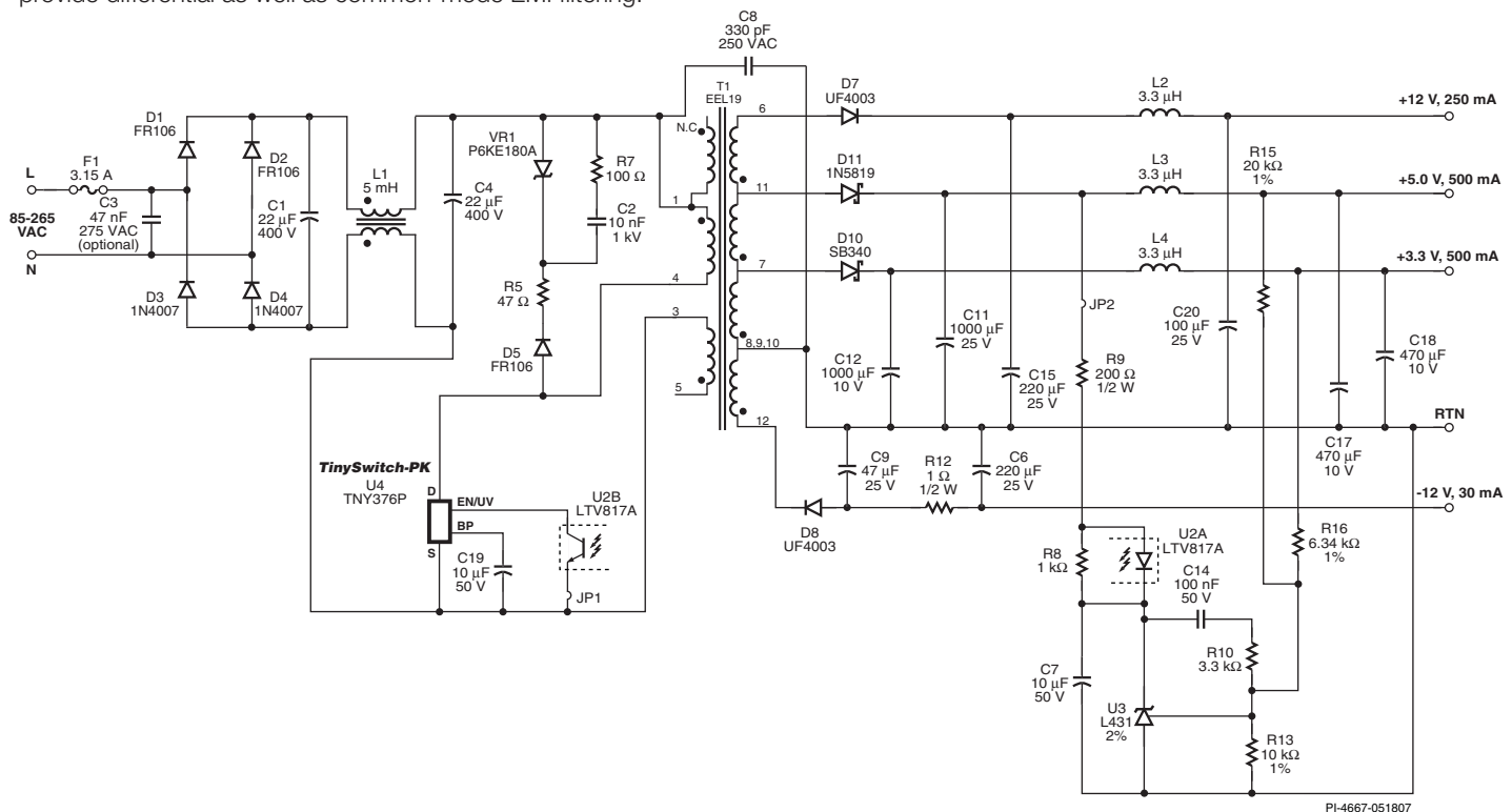
Figure 1. Schematic of a Universal Input, and Multiple-Output DVD Player Power Supply.
