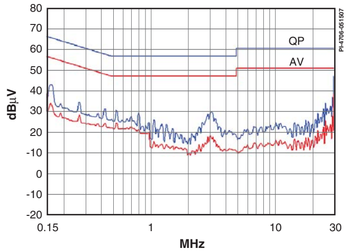
Figure 3. Conducted EMI at 230 VAC with Output Grounded (CISPR-22 Limit Lines Shown).
