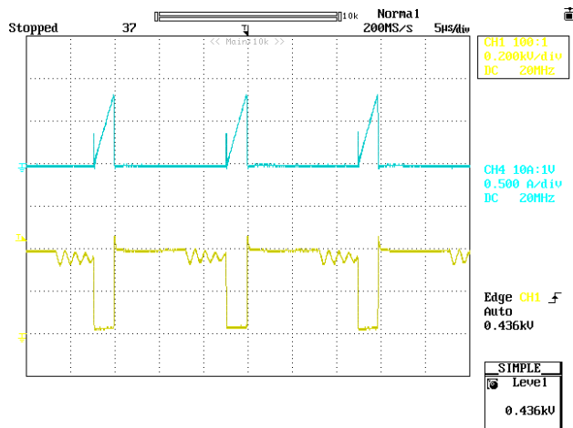
Figure 23 – 265 VAC, Full Load. Upper: I_{DRAIN} , 0.5 A / div. Lower: V_{DRAIN} , 200 V / div., 5 µs / div.
