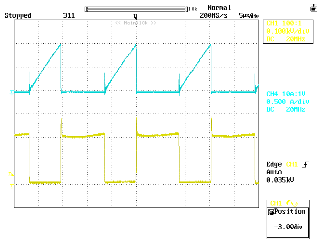
Figure 22 – 90 VAC, Full Load. Upper: I_{DRAIN} , 0.5 A / div. Lower: V_{DRAIN} , 100 V, 5 µs / div.
