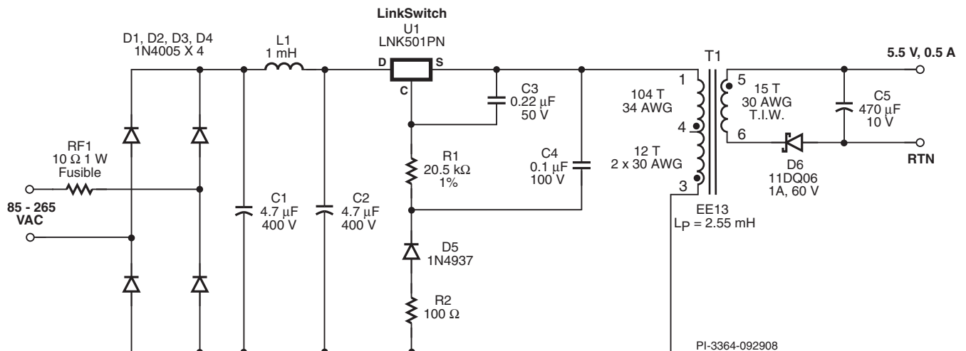
Figure 1. LinkSwitch 2.75 W Charger Power Supply.
