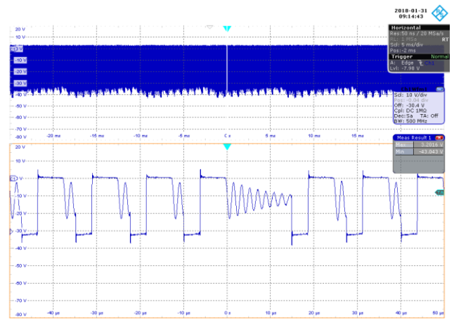
Figure 77 – 115 VAC 60 Hz, Full Load. CH1: V FWL_Diode - 10 V / div., 5 ms / div. Zoom: 10 μs / div. PIV MAX = 43.043 V.
