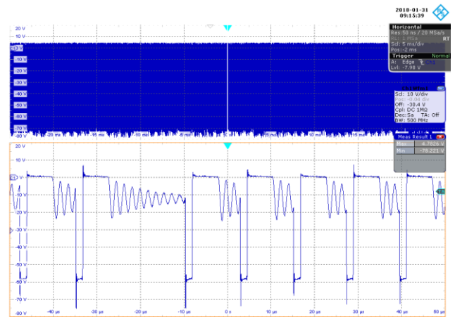
Figure 79 – 265 VAC 50 Hz, Full Load. CH1: V FWL_Diode - 10 V / div., 5 ms / div. Zoom: 10 μs / div. PIV MAX = 78.221 V.
