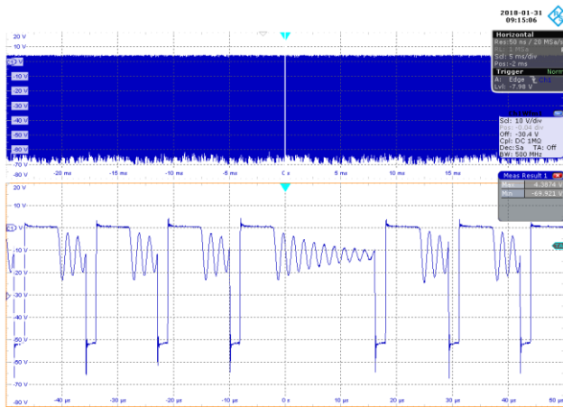
Figure 78 – 230 VAC 50 Hz, Full Load. CH1: V FWL_Diode - 10 V / div., 5 ms / div. Zoom: 10 μs / div. PIV MAX = 69.921 V.
