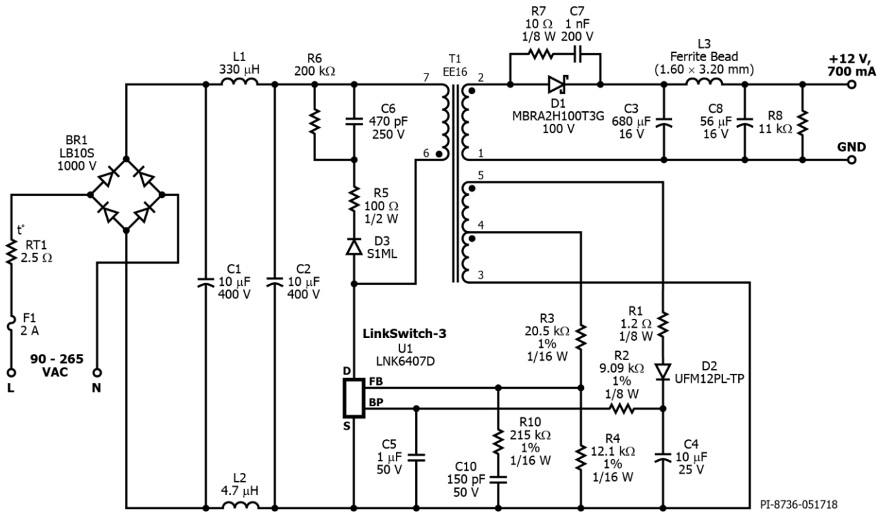
Figure 3 – Schematic Diagram.
